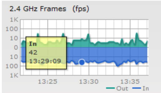
Figure 185 - 2.4 GHz Management Frames (fps) Graph
